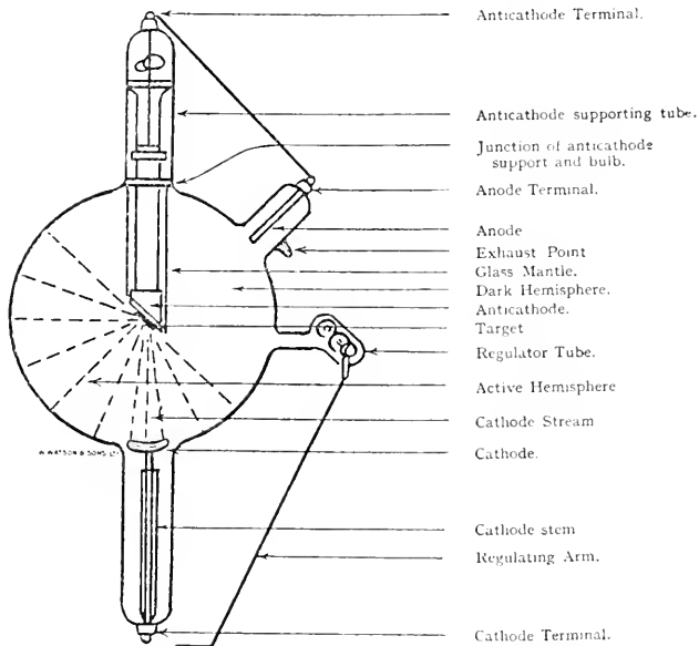
FIG. 25.—Diagram of an X-ray tube with parts named, showing the paths of the cathode stream from the cathode impinging on the anti-cathode; the active hemisphere shows the paths of most of the X-rays generated. (Watson).
